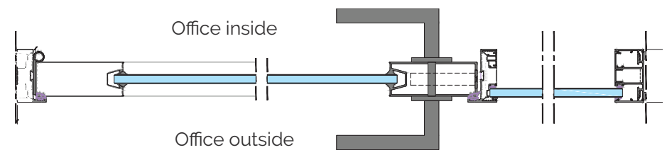
Horizontal Section / 'SUMMIT' Singled Glazed Partition w/ "Entry" Door
