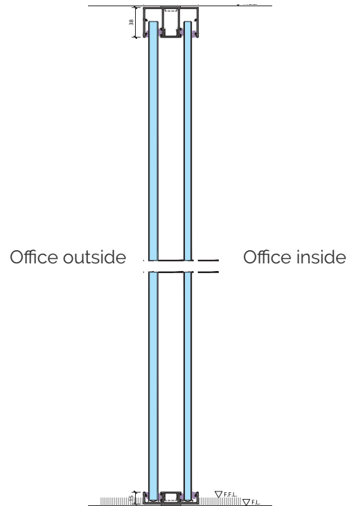
Vertical Section / Double Glazed Partition
