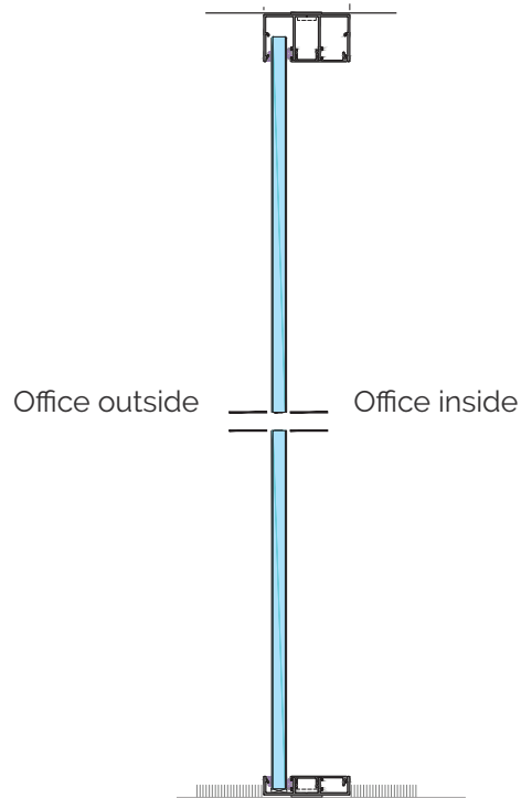
Vertical Section / Single Glazed Partition
