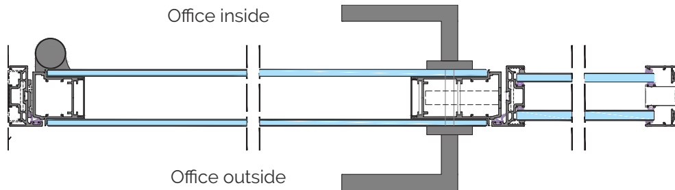
Horizontal Section / 'SUMMIT' Double Glazed Partition w/ "PLUS" Door
