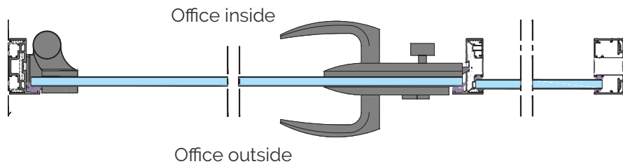
Horizontal Section / 'SUMMIT' Singled Glazed Partition w/ Frameless Single Glazed Door
