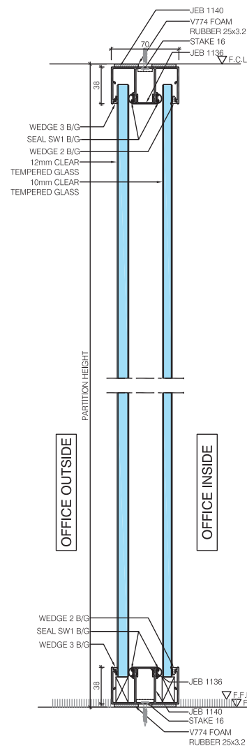
V01 VERTICAL SECTION DOUBLE GLAZED PARTITION
