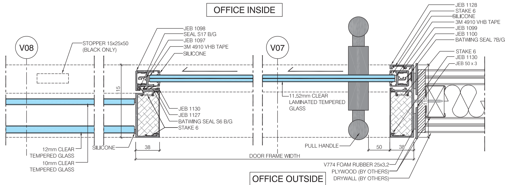
H05 HORIZONTAL SECTION DOUBLE GLAZED PARTITION w/ SINGLE GLAZED SLIDING DOOR
