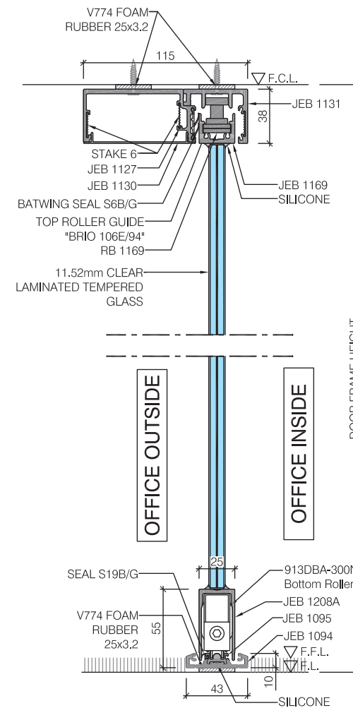
V07 VERTICAL SECTION SINGLE GLAZED SLIDING DOOR
