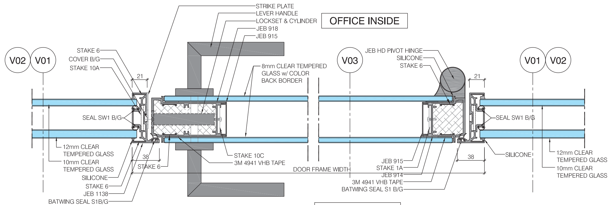
H03 HORIZONTAL SECTION DOUBLE GLAZED PARTITION w/ DOUBLE GLAZED DOOR
