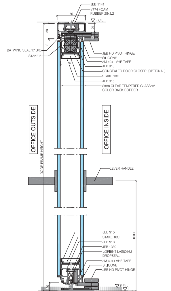
V03 VERTICAL SECTION DOUBLE GLAZED DOOR
