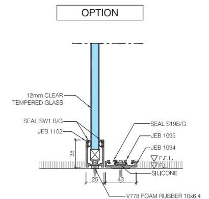
V05A VERTICAL SECTION SLIDING DOOR SIDELIGHT w/ 38mm HEIGHT BOTTOM CHANNEL
