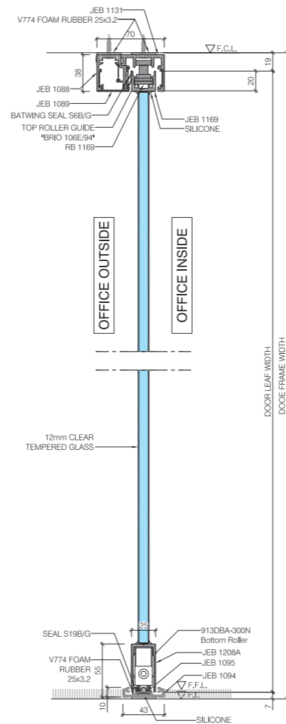
V04 VERTICAL SECTION SINGLE GLAZED SLIDING DOOR
