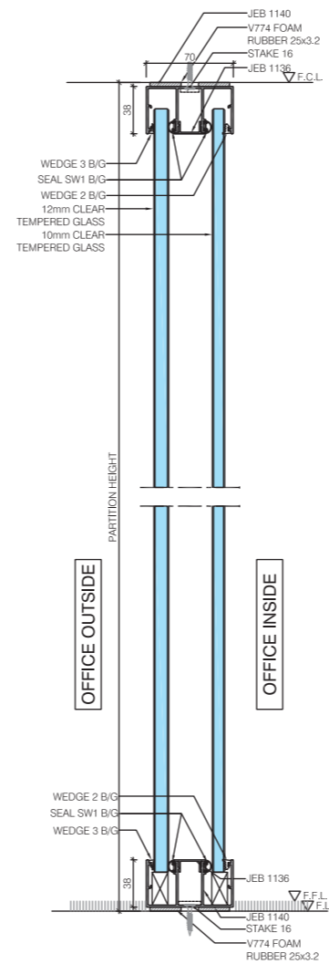
V01 VERTICAL SECTION DOUBLE GLAZED PARTITION
