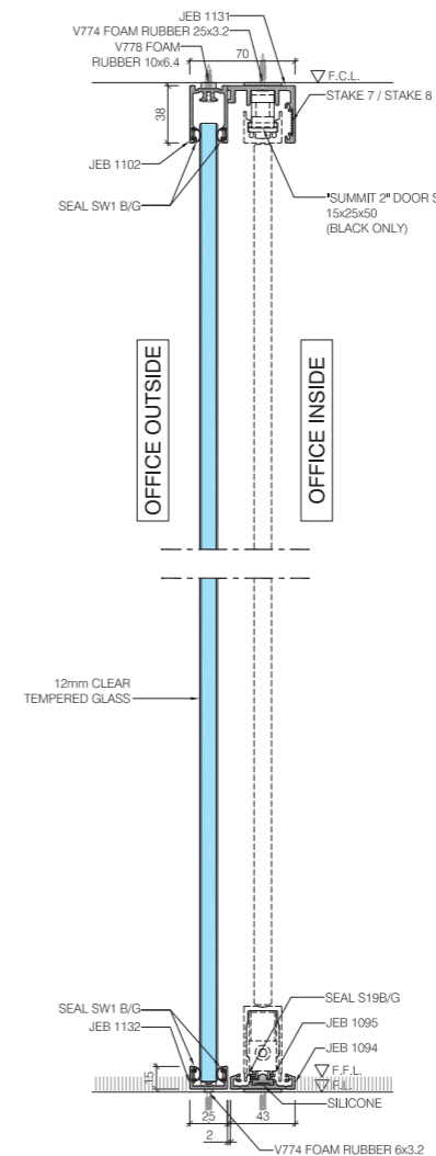
V05 VERTICAL SECTION SLIDING DOOR SIDELIGHT w/ 15mm HEIGHT BOTTOM CHANNEL
