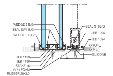
V08 VERTICAL SECTION SLIDING DOOR SIDELIGHT w/ DOUBLE GLAZED PARTITION
