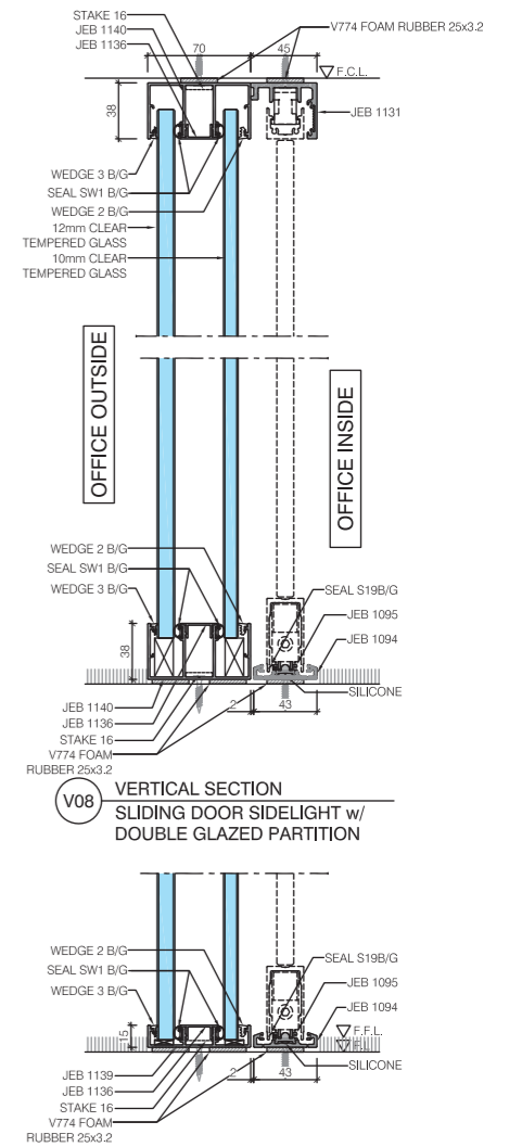
V08 VERTICAL SECTION SLIDING DOOR SIDELIGHT w/ DOUBLE GLAZED PARTITION
