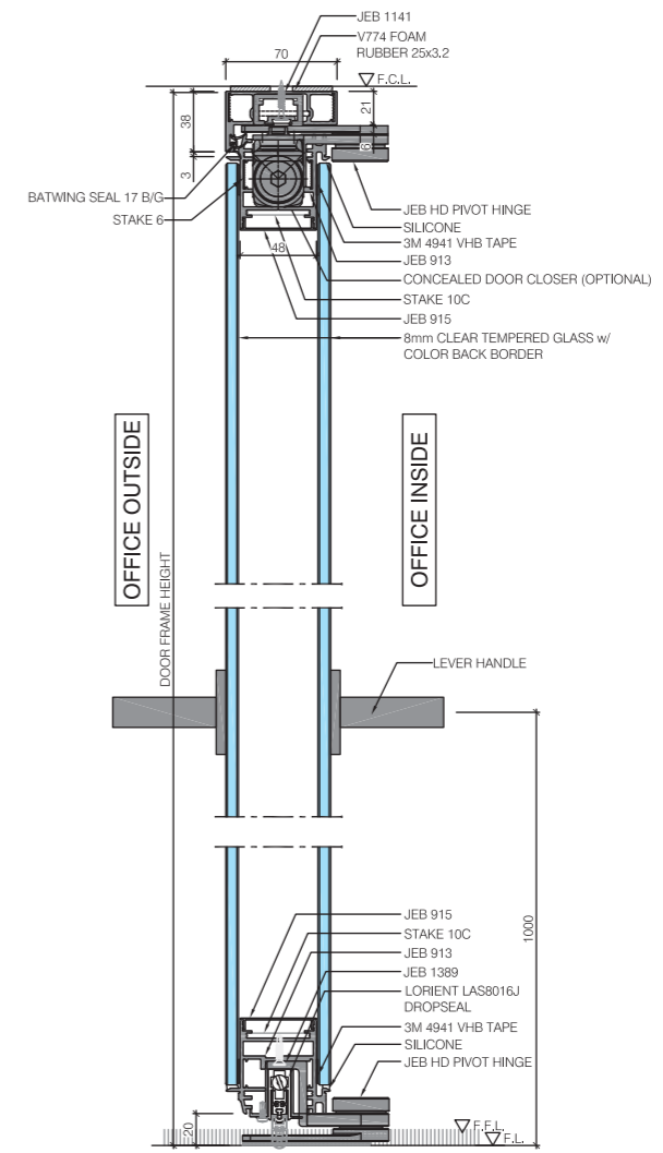
V03 VERTICAL SECTION DOUBLE GLAZED DOOR
