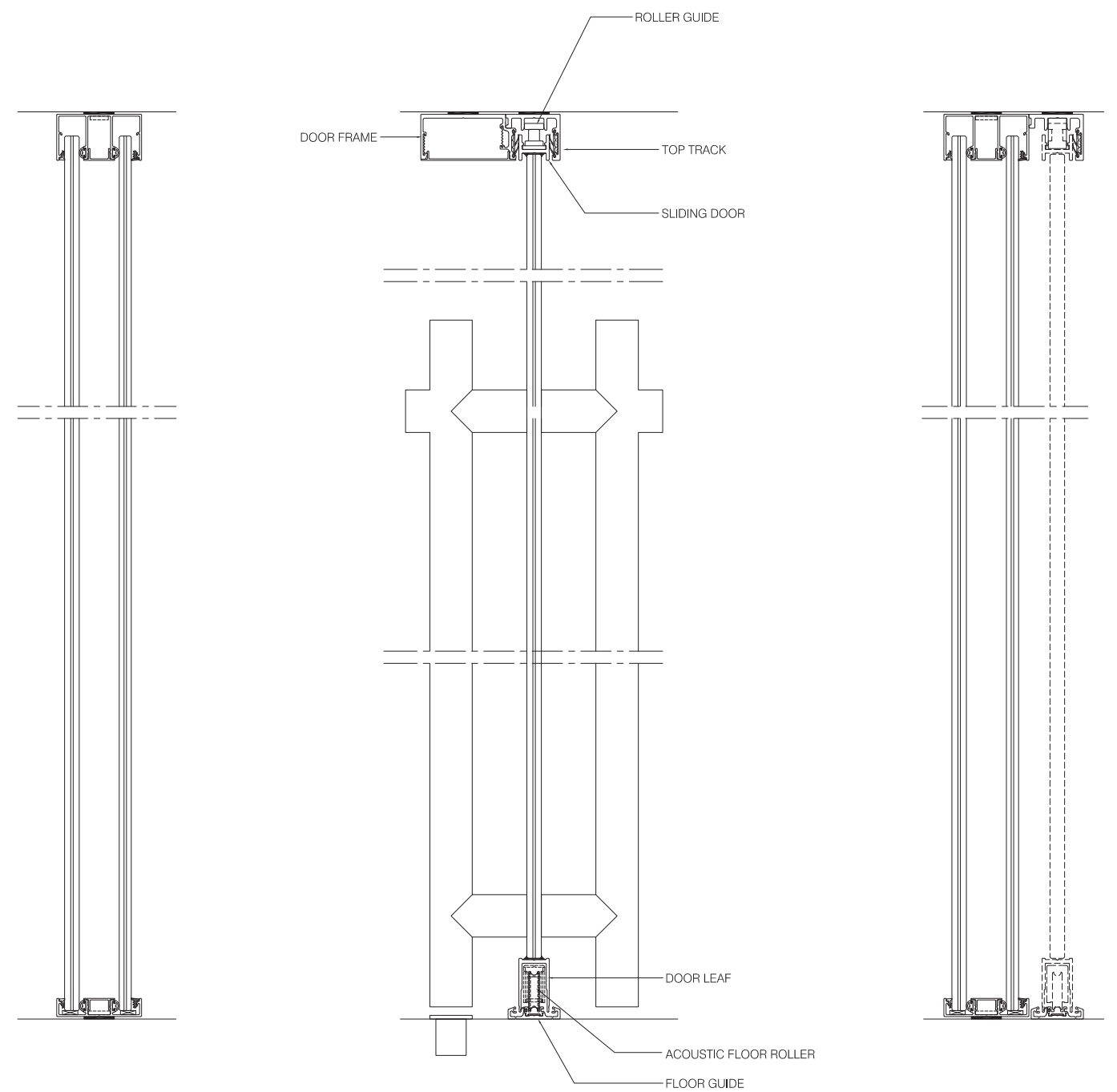
VERTICAL SECTION
