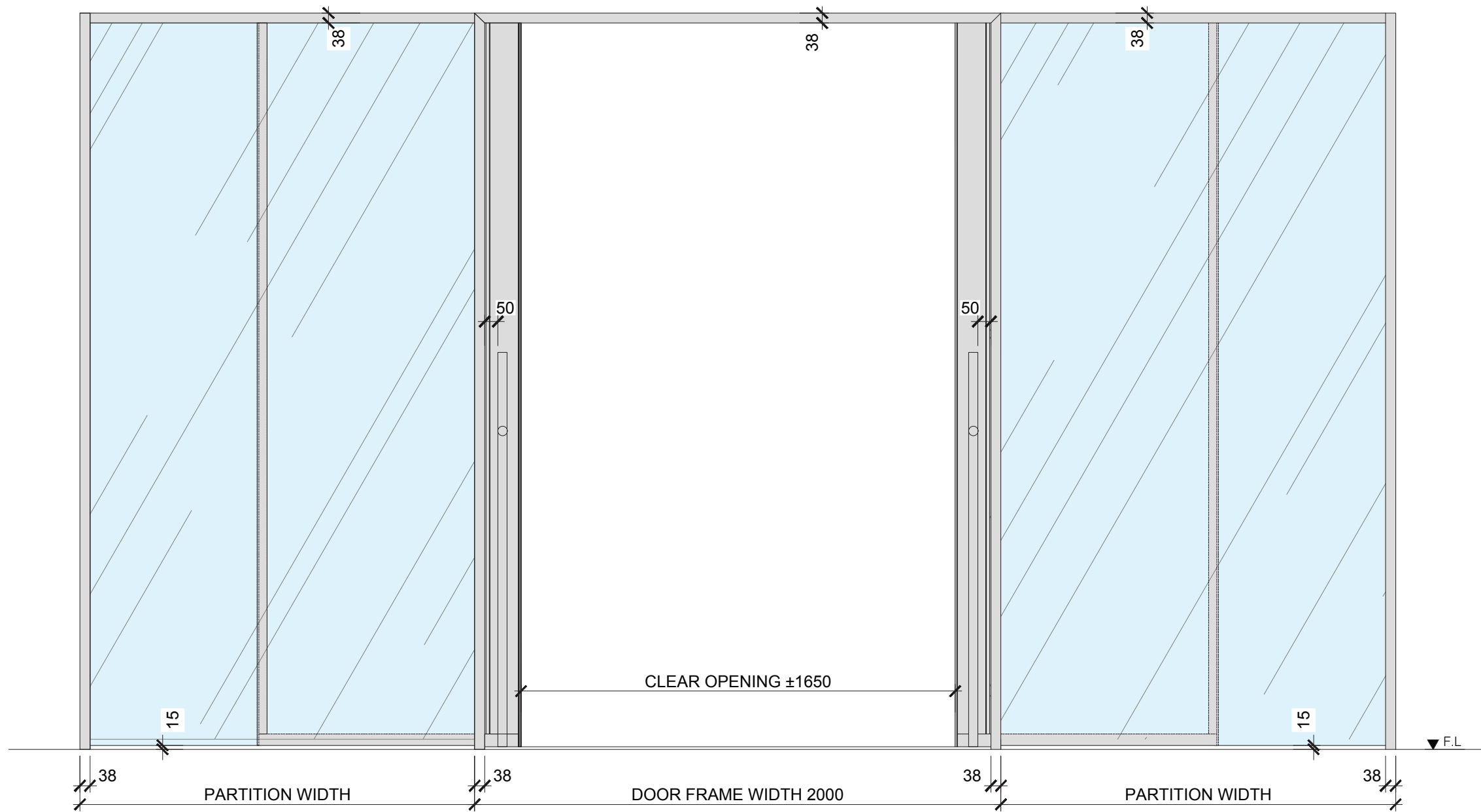
E01 ELEVATION DOUBLE SLIDING DOOR w/ SIDE LIGHT
