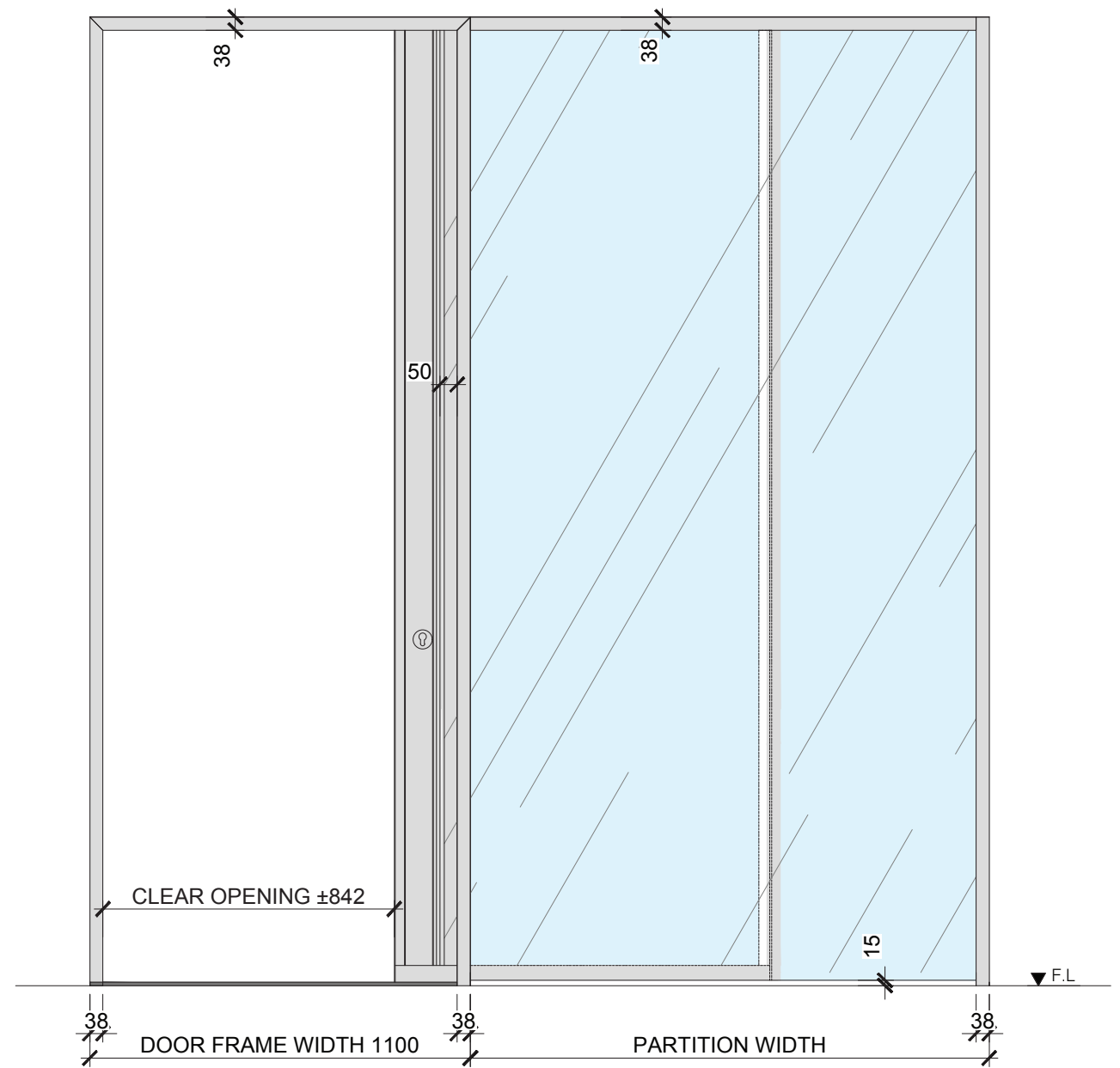
E01A ELEVATION SLIDING DOOR w/ SIDE LIGHT
