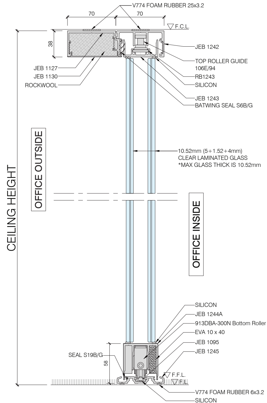
V01 VERTICAL SECTION DOUBLE GLAZED SLIDING DOOR
