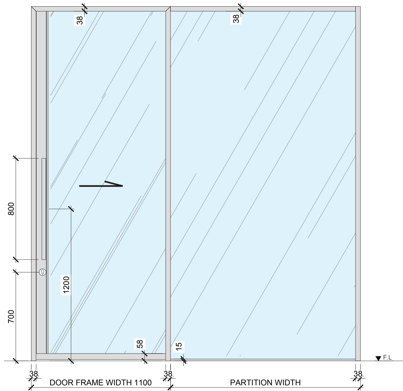
E02 ELEVATION SLIDING DOOR w/ SIDE LIGHT (PULL HANDLE)
