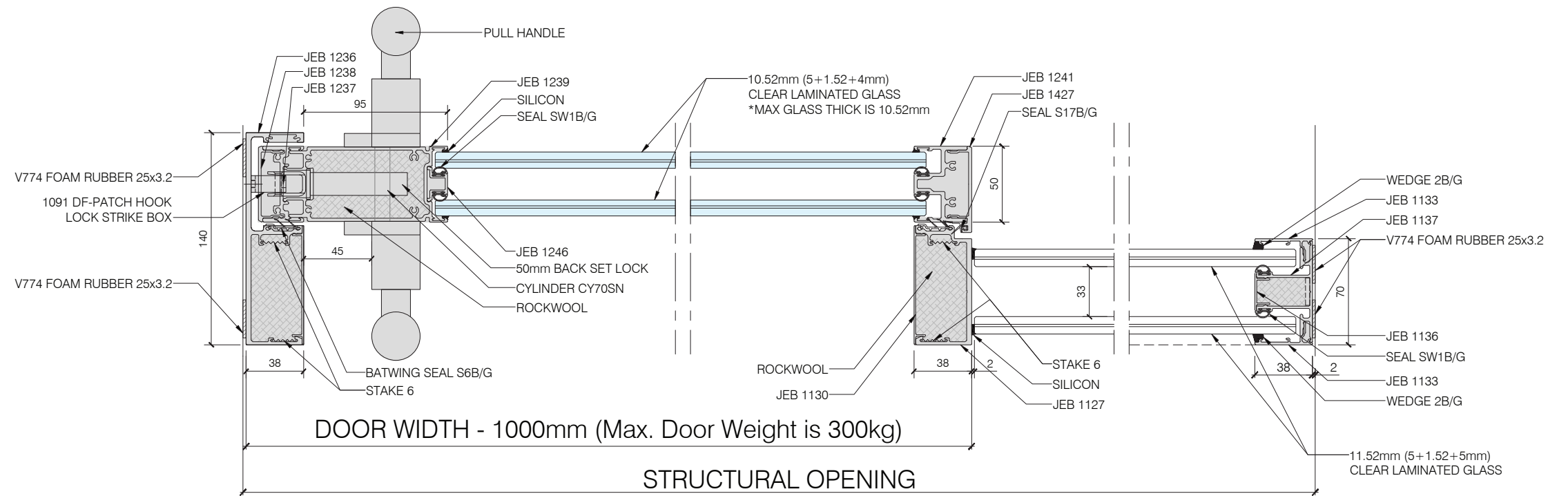
H01 HORIZONTAL SECTION DOUBLE GLAZED SLIDING DOOR W/ DOUBLE GLAZED PARTITION (PULL HANDLE)
