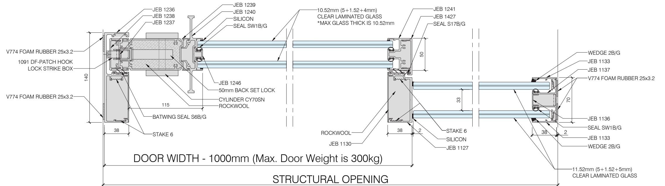
H01 HORIZONTAL SECTION DOUBLE GLAZED SLIDING DOOR W/ DOUBLE GLAZED PARTITION
