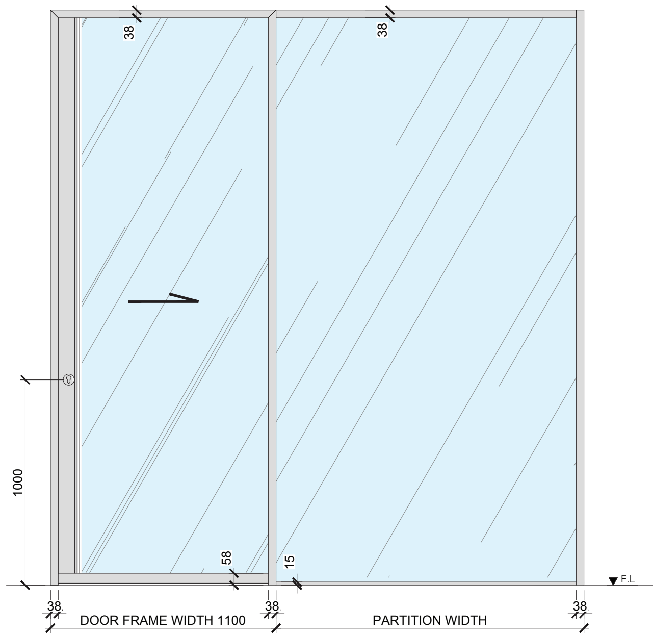
E01 ELEVATION SLIDING DOOR w/ SIDE LIGHT
