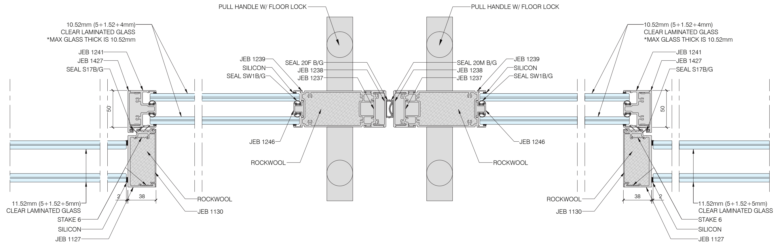
H02 HORIZONTAL SECTION DOUBLE GLAZED DOUBEL SLIDING DOOR W/ DOUBLE GLAZED PARTITION
