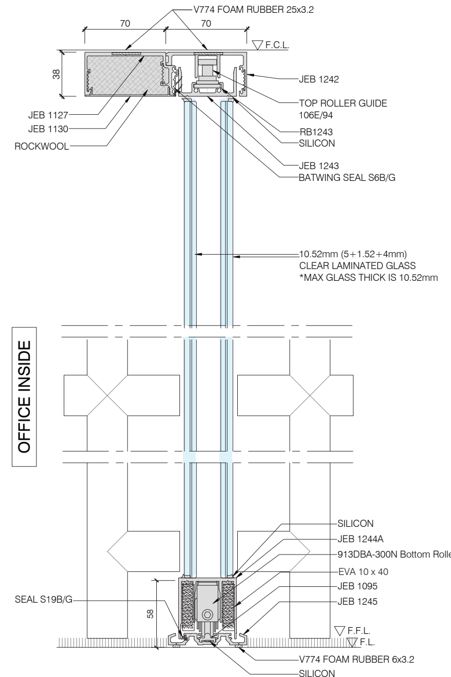
V01 VERTICAL SECTION DOUBLE GLAZED SLIDING DOOR (PULL HANDLE)
