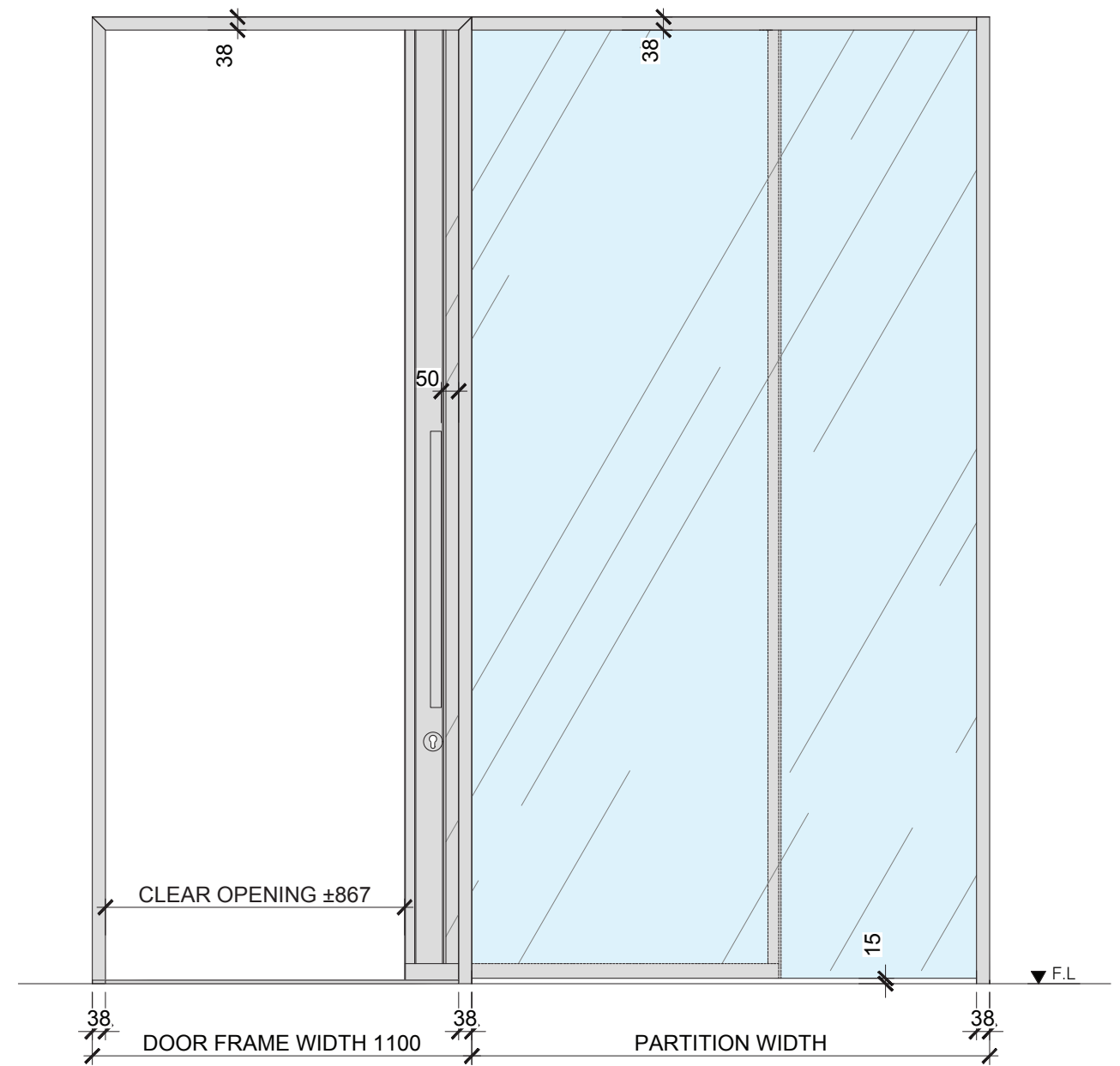
E02A ELEVATION SLIDING DOOR w/ SIDE LIGHT (PULL HANDLE)
