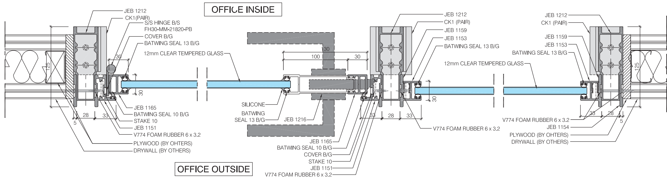
H01 HORIZONTAL SECTION SINGLE GLAZED PARTITION W\ SINGLE GLAZED DOOR
