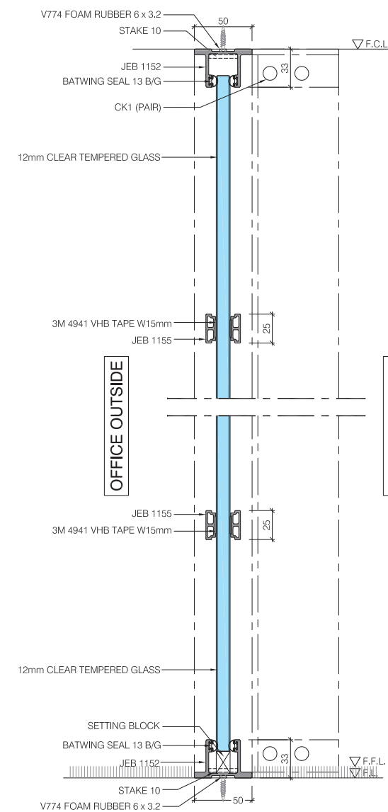
V01 VERTICAL SECTION SINGLE GLAZED PARTITION
