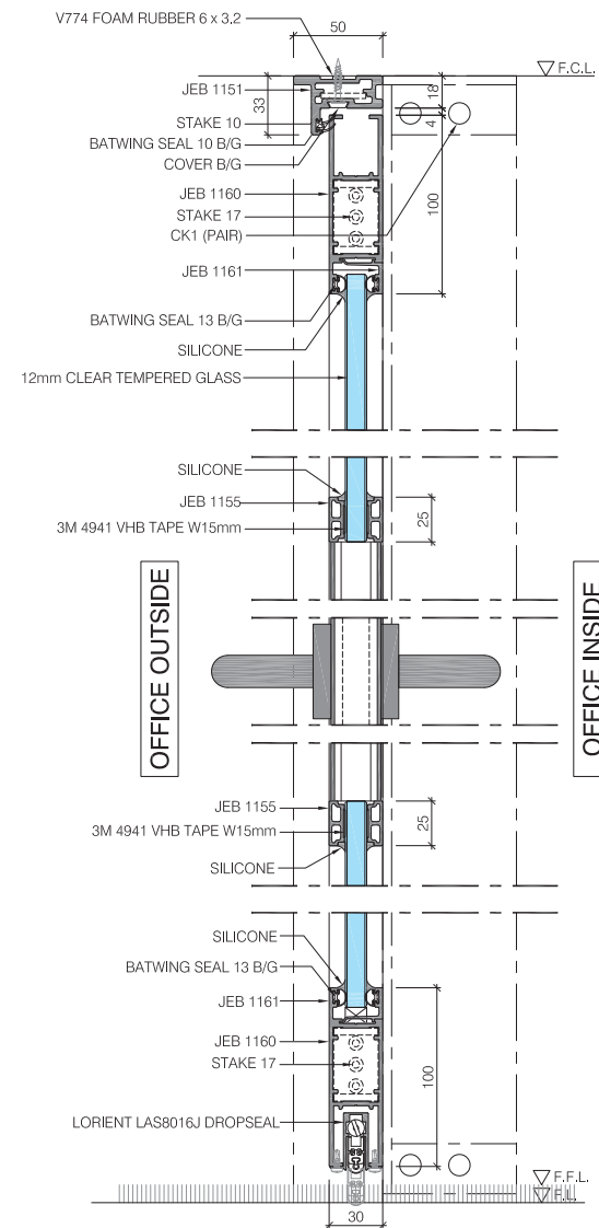
V02 VERTICAL SECTION SINGLE GLAZED DOOR
