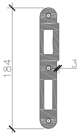
Art: 1151 DF STRIKE PLATE (REVERSIBLE)
