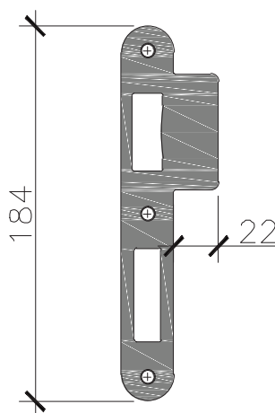
Art: 1138 DF STRIKE PLATE (REVERSIBLE)
