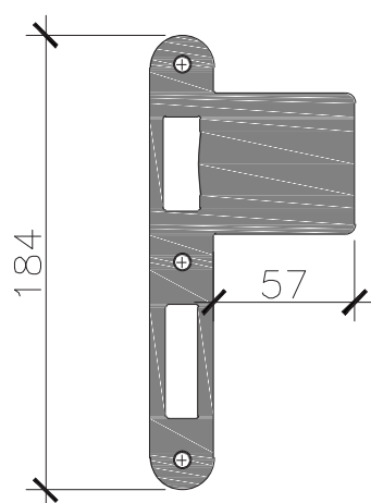
Art: 1027A /892A DF STRIKE PLATE (REVERSIBLE)
