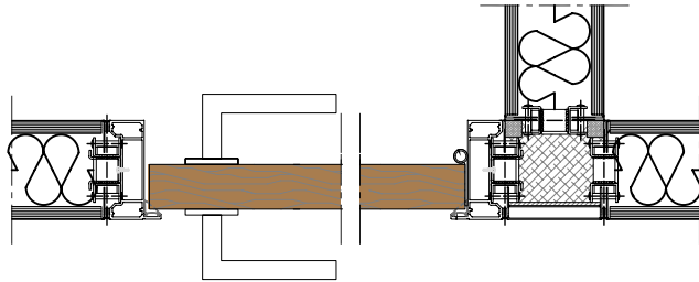
Glazed T-join (Timber Door)
