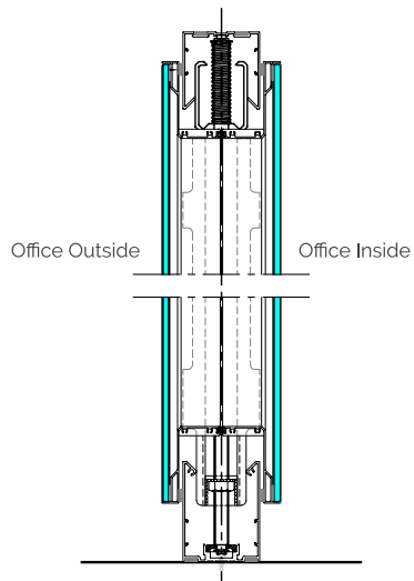
Vertical Section / Double Glazed Panel
