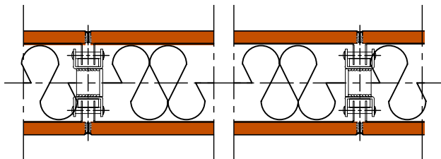
Horizontal Section / Fabric Panel
