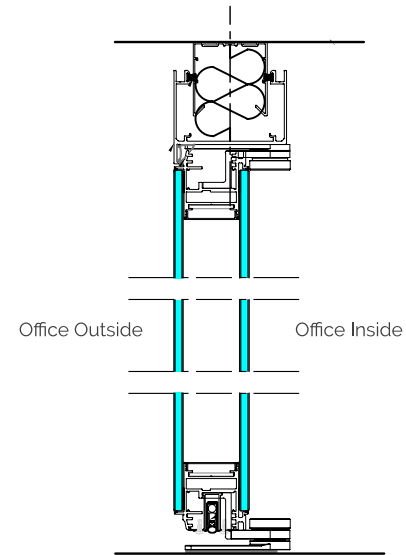
Vertical Section / Double Glazed Door
