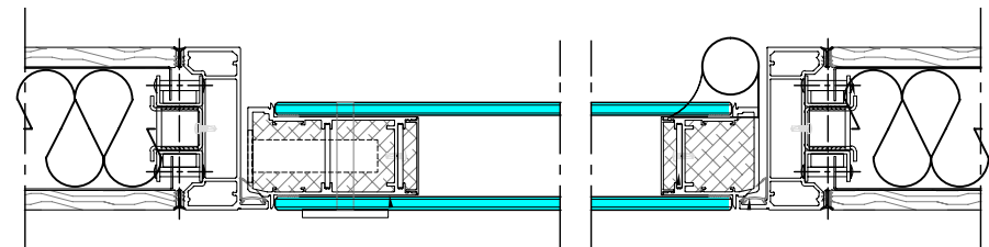
Horizontal Section / Double Glazed Door
