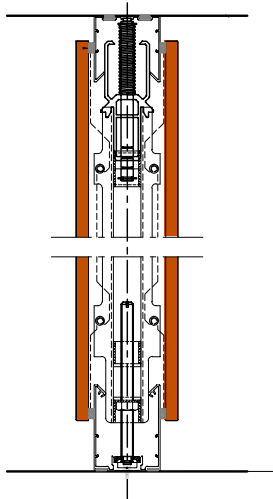
Vertical Section / Fabric Panel
