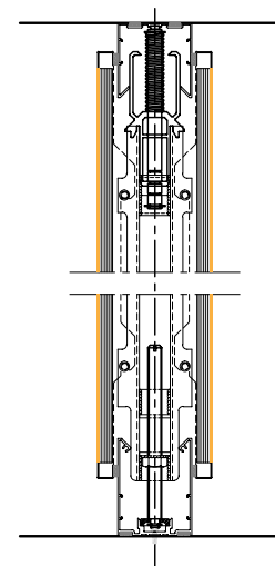
Vertical Section / Metal Panel
