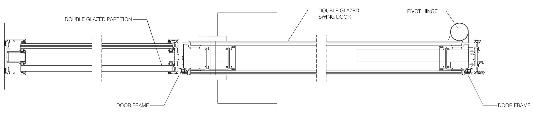
HORIZONTAL SECTION
