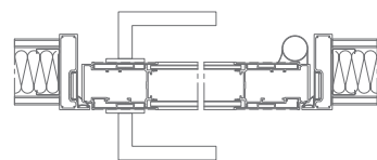
Double Glazed 66mm with Veneer Inlays
