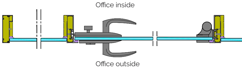
Horizontal Section / Singled Glazed Partition w/ Frameless Single Glazed Door
